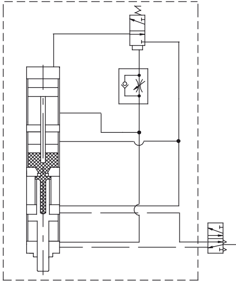
Pneumatic System
